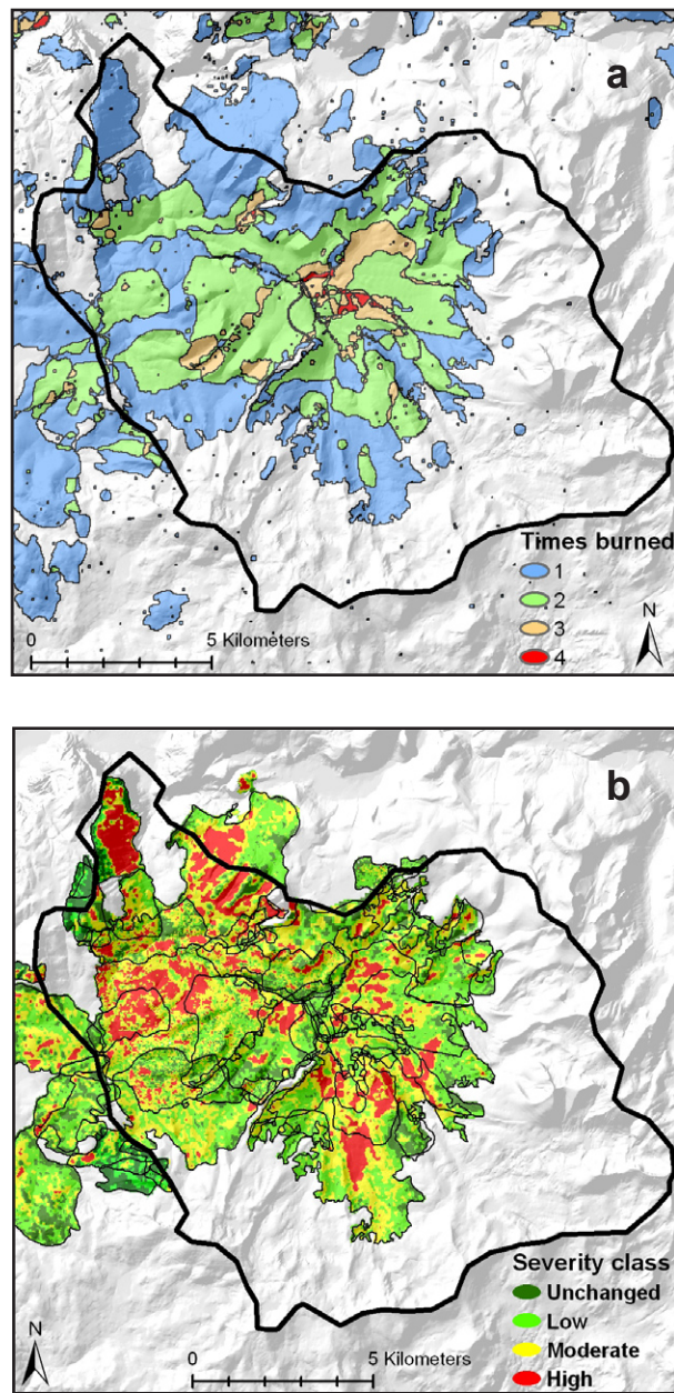
Figure 3. Fires in the Illilouette Creek basin burned to form a jigsaw pattern where some fires were limited by previous fires while others reburned extensive areas (a). The number of times burned is indicated for 28 fires greater than 40 ha from 1973 through 2011. Composite fire severity for the 28 fires greater than 40 ha in the Illilouette Creek basin from 1973 through 2011 (b). The severity of the last fire to burn an area is shown in colors, and perimeters for all 28 fires are shown in black.
